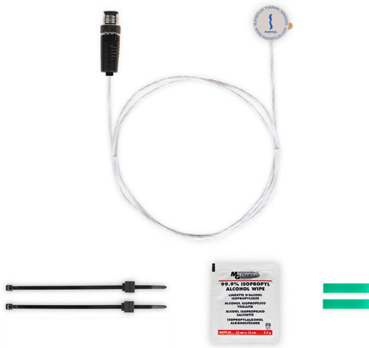
Figure 3 PVMT01 measures the PV module temperature. The Pt1000 sensor is incorporated in a small aluminium disk and supplied with 2 x solar clips, 2 x polyester tapes and a pre-saturated IPA wipe.
