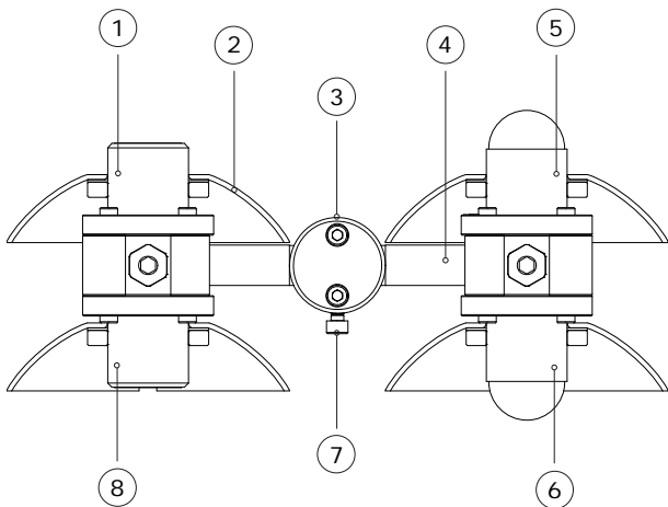
Figure 3 overview of NR01: (1) upfacing pyrgeometer, (2) sun screens, (3,4,7) levelling assembly for x- and y-axis, (5) upfacing pyranometer, (6) downfacing pyranometer, (8) downfacing pyrgeometer
